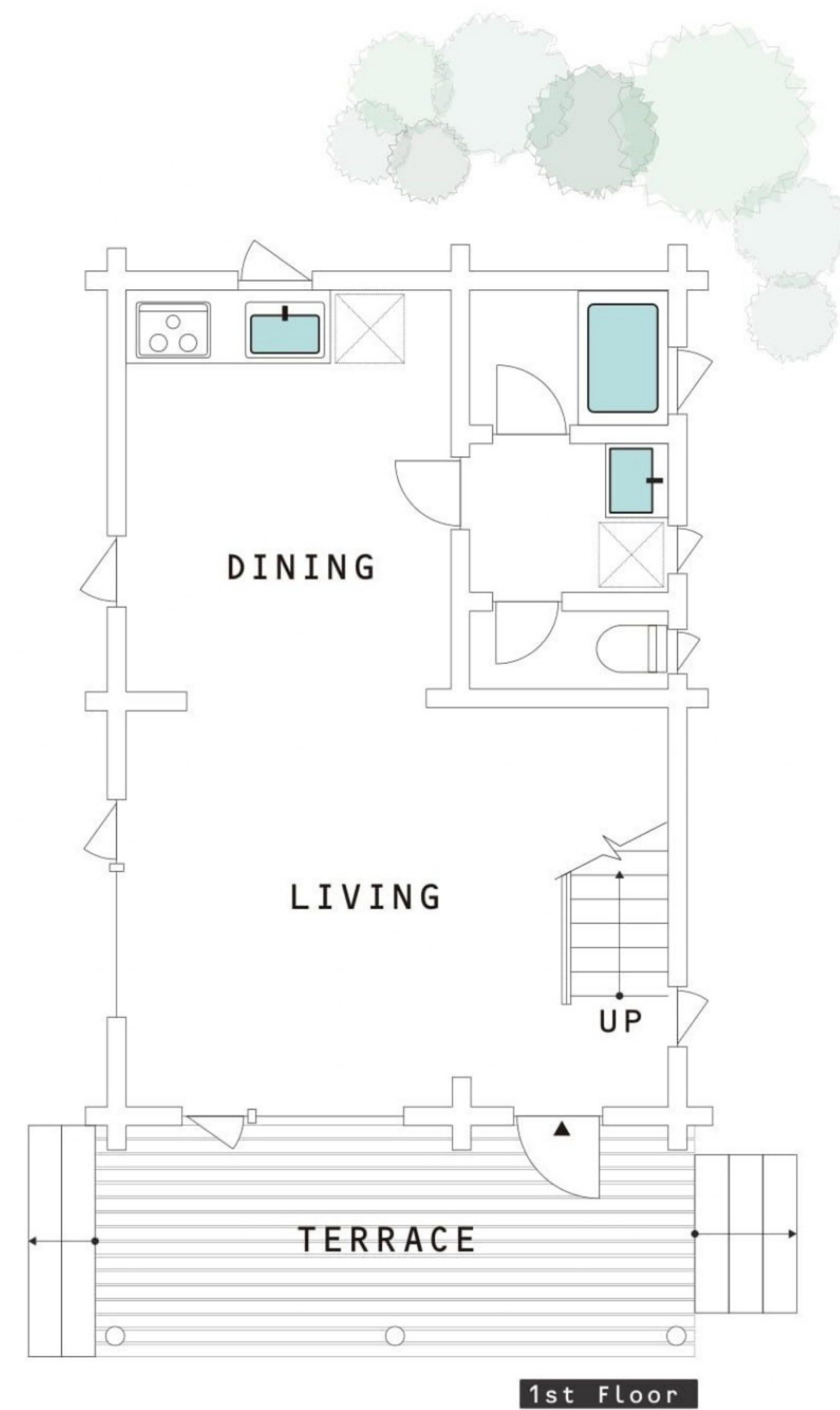
1st Floor
